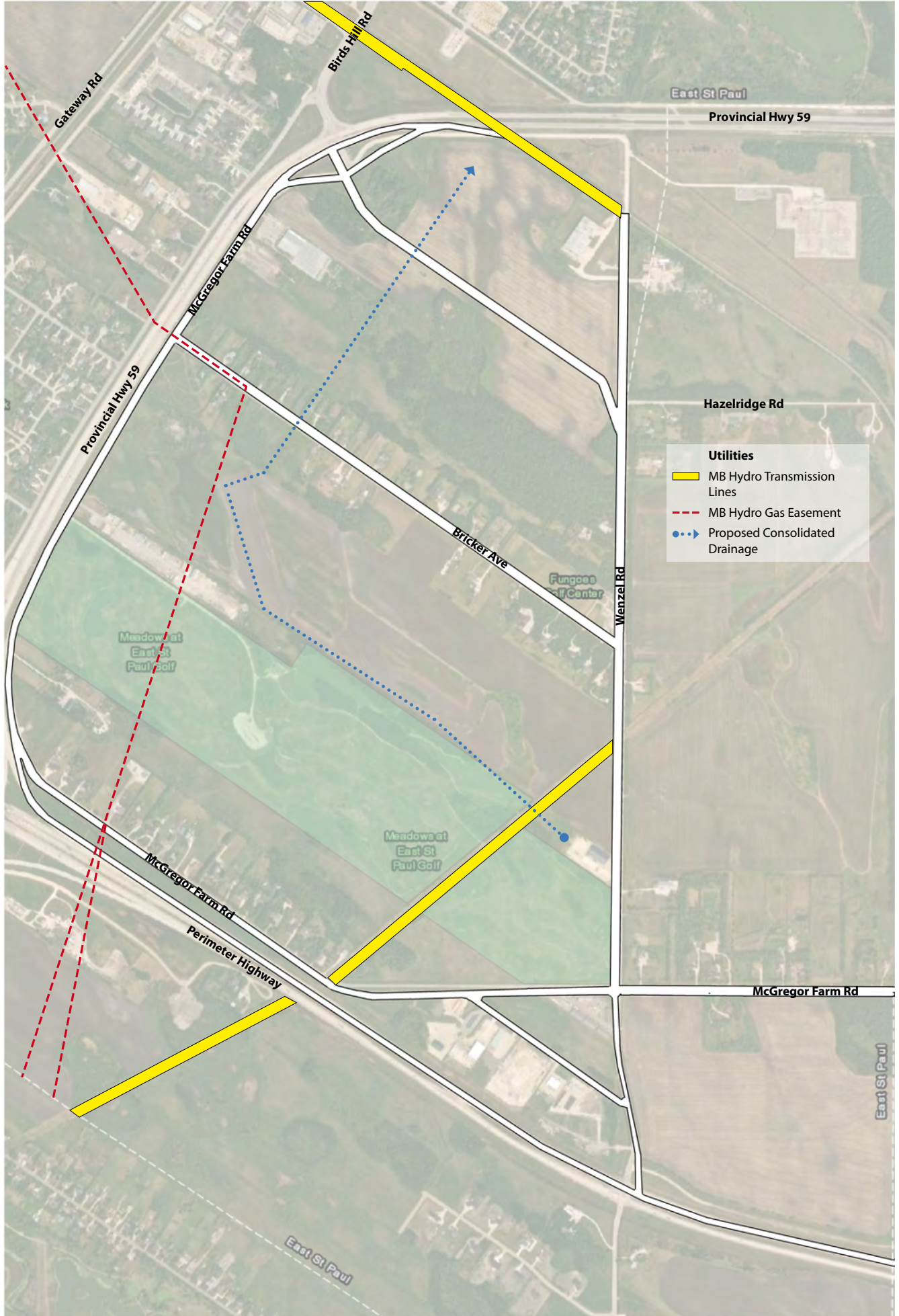
Figure 43. Utility corridors
