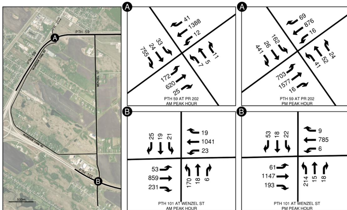
Figure 6: Pre-Development Volumes – 2036 AM and PM Peak Hours
