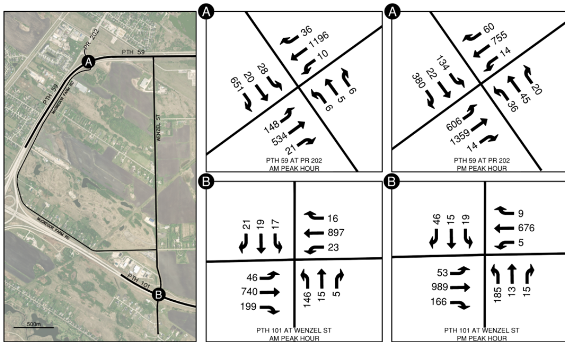
Figure 5: Pre-Development Volumes – 2026 AM and PM Peak Hours
